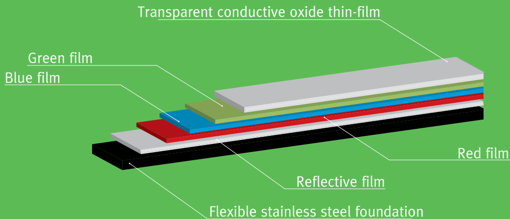
Profile of photovoltaic module
